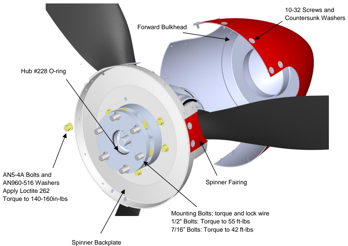
Figure 3. Spinner Assembly
