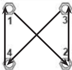
Figure5- GA-UL260 4-Bolt Tightening Pattern Continued on Pg.11
