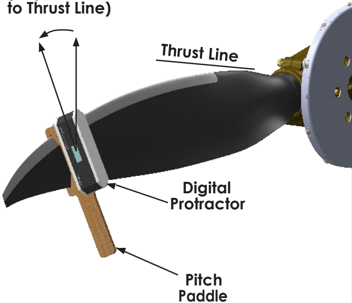
Figure 4- GA-UL260 Pitch Paddle
